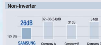
*Lowest noise level of an indoor unit for Non-Inverter / R410A / Heat Pump
