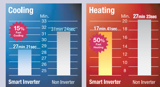
Time to cool from 33°C to 25°C
